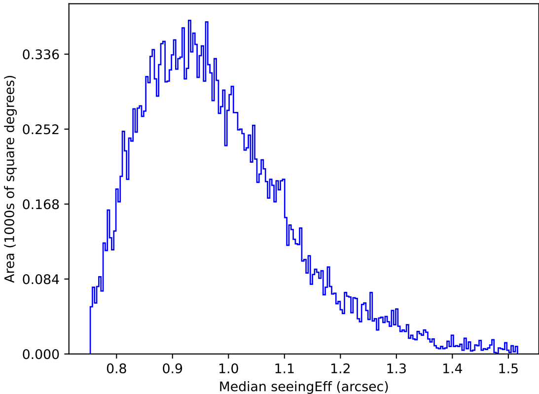
too_elab_r32_d2_gz_v3.4_10yrs Yr 1 z band: Median seeingEff
