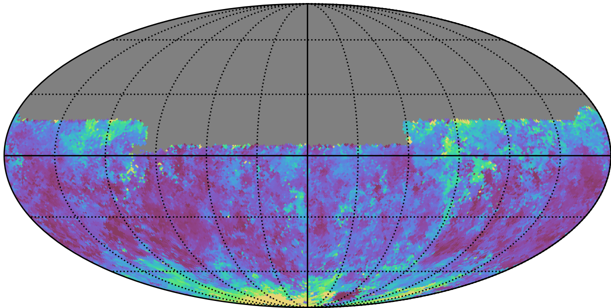
too_elab_r32_d2_gz_v3.4_10yrs Yr 1 y band: Median seeingEff
