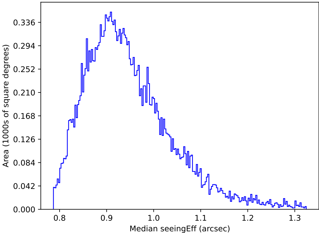
too_elab_r32_d2_gz_v3.4_10yrs Yr 1 y band: Median seeingEff
