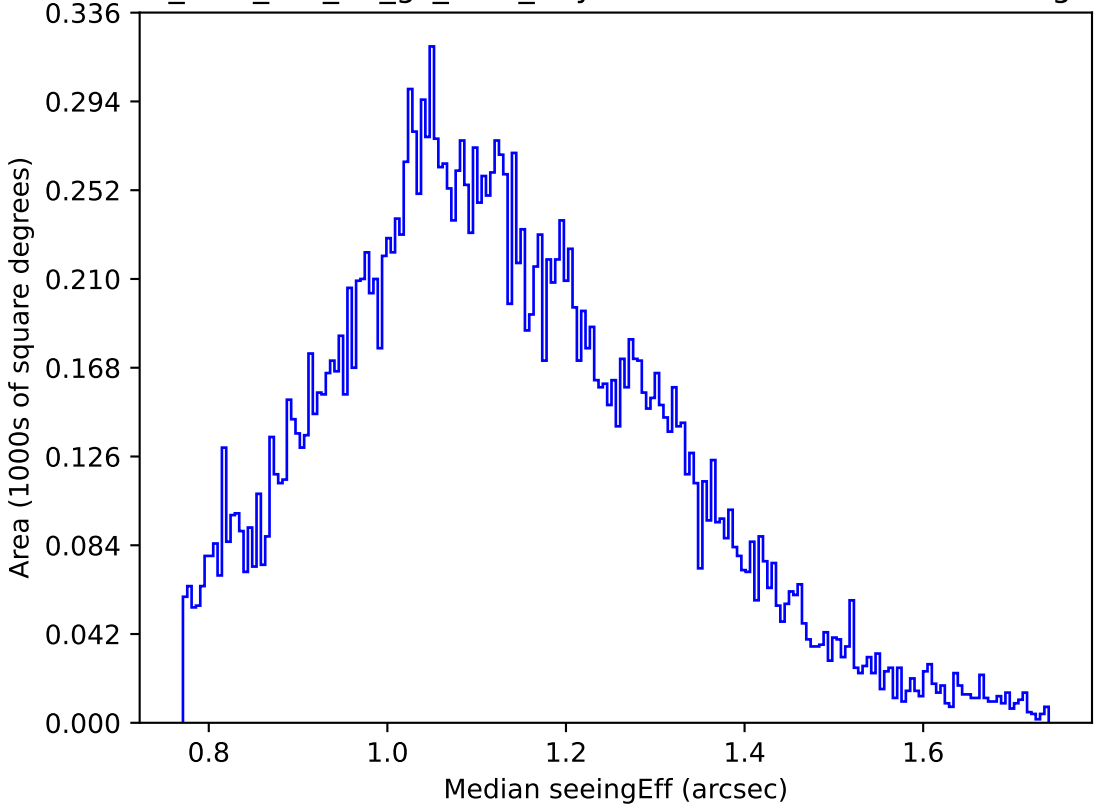
too_elab_r32_d2_gz_v3.4_10yrs Yr 1 u band: Median seeingEff
