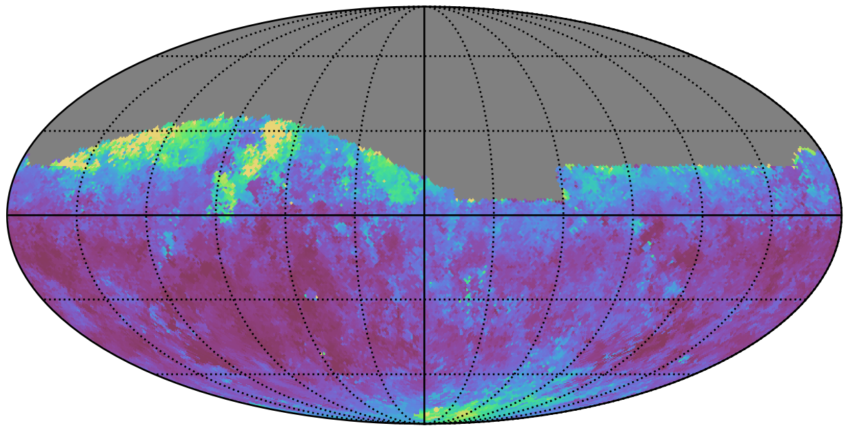
too_elab_r32_d2_gz_v3.4_10yrs Yr 1 i band: Median seeingEff
