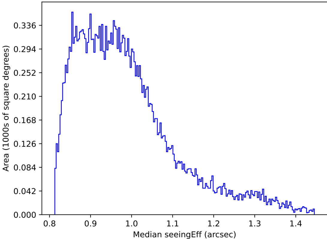
too_elab_r32_d2_gz_v3.4_10yrs Yr 1 all bands: Median seeingEff
