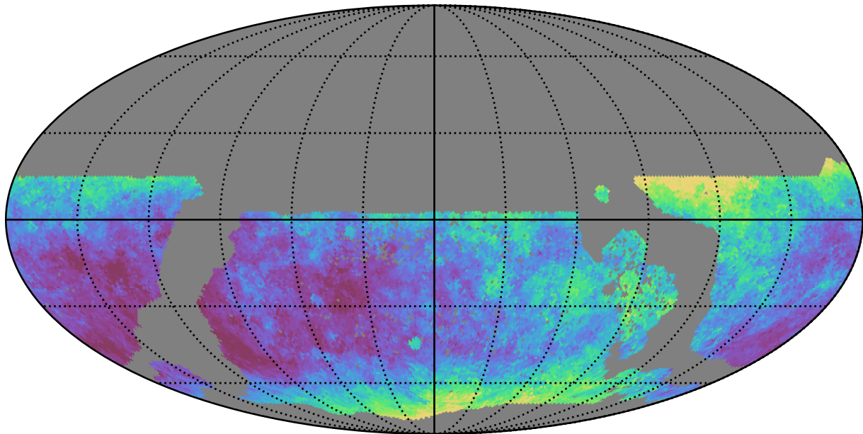
too_elab_r32_d2_gz_v3.4_10yrs WFD y band: Median seeingEff
