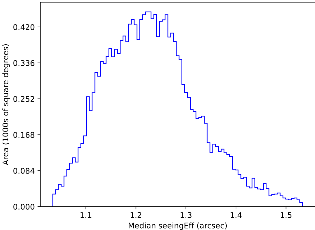
too_elab_r32_d2_gz_v3.4_10yrs WFD u band: Median seeingEff
