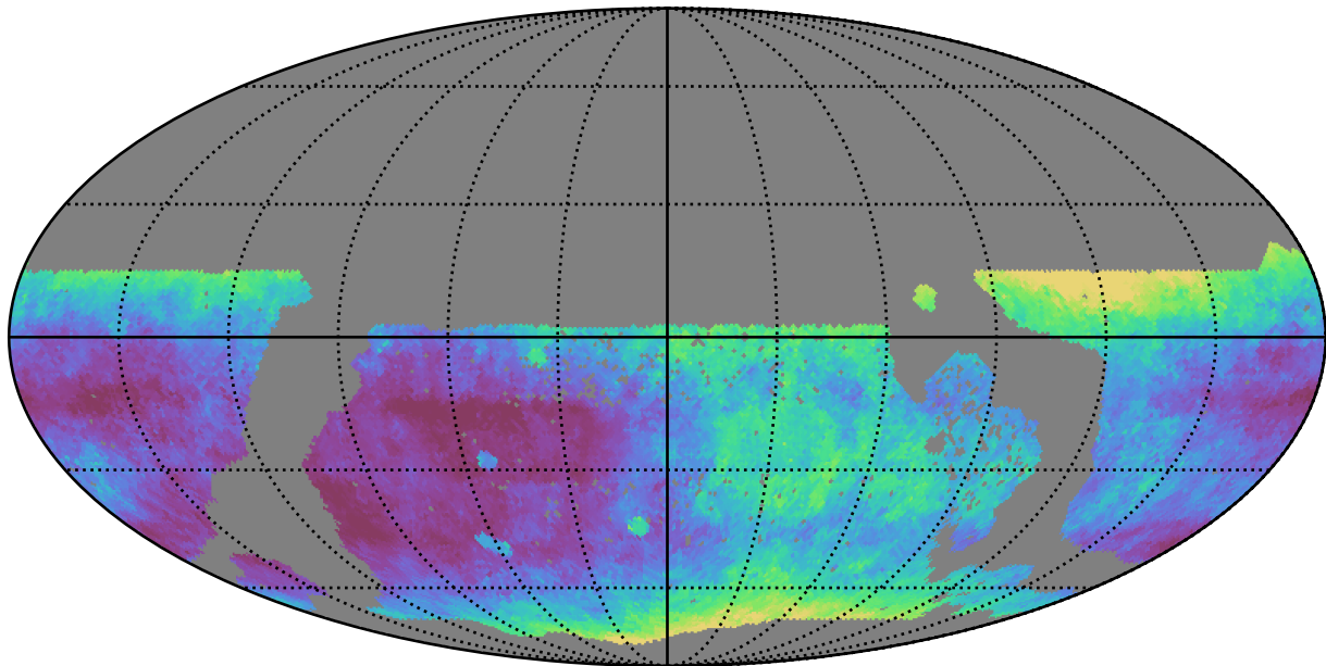
too_elab_r32_d2_gz_v3.4_10yrs WFD r band: Median seeingEff
