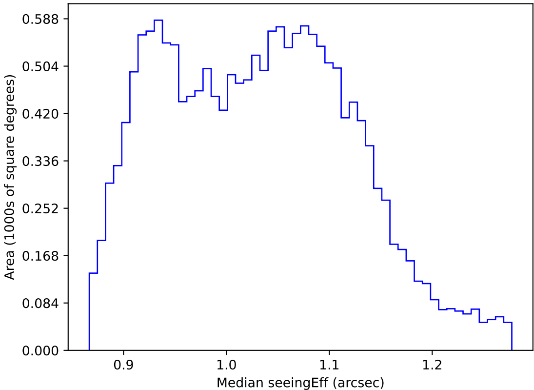
too_elab_r32_d2_gz_v3.4_10yrs WFD r band: Median seeingEff
