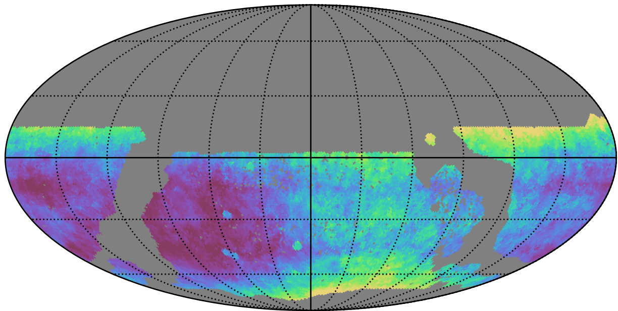
too_elab_r32_d2_gz_v3.4_10yrs WFD i band: Median seeingEff
