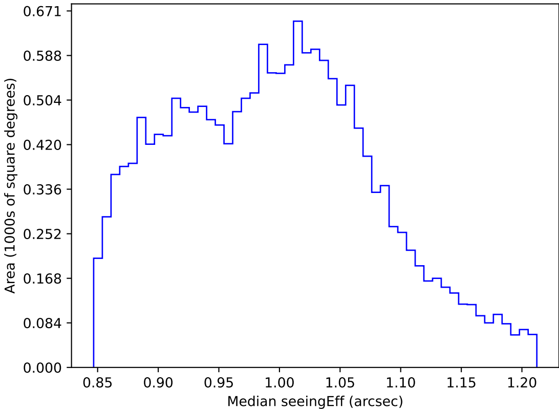
too_elab_r32_d2_gz_v3.4_10yrs WFD i band: Median seeingEff
