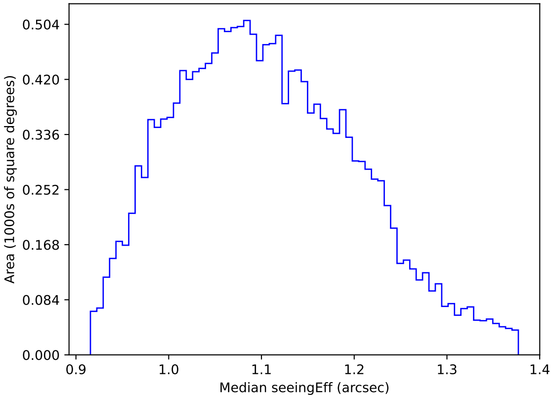
too_elab_r32_d2_gz_v3.4_10yrs WFD g band: Median seeingEff
