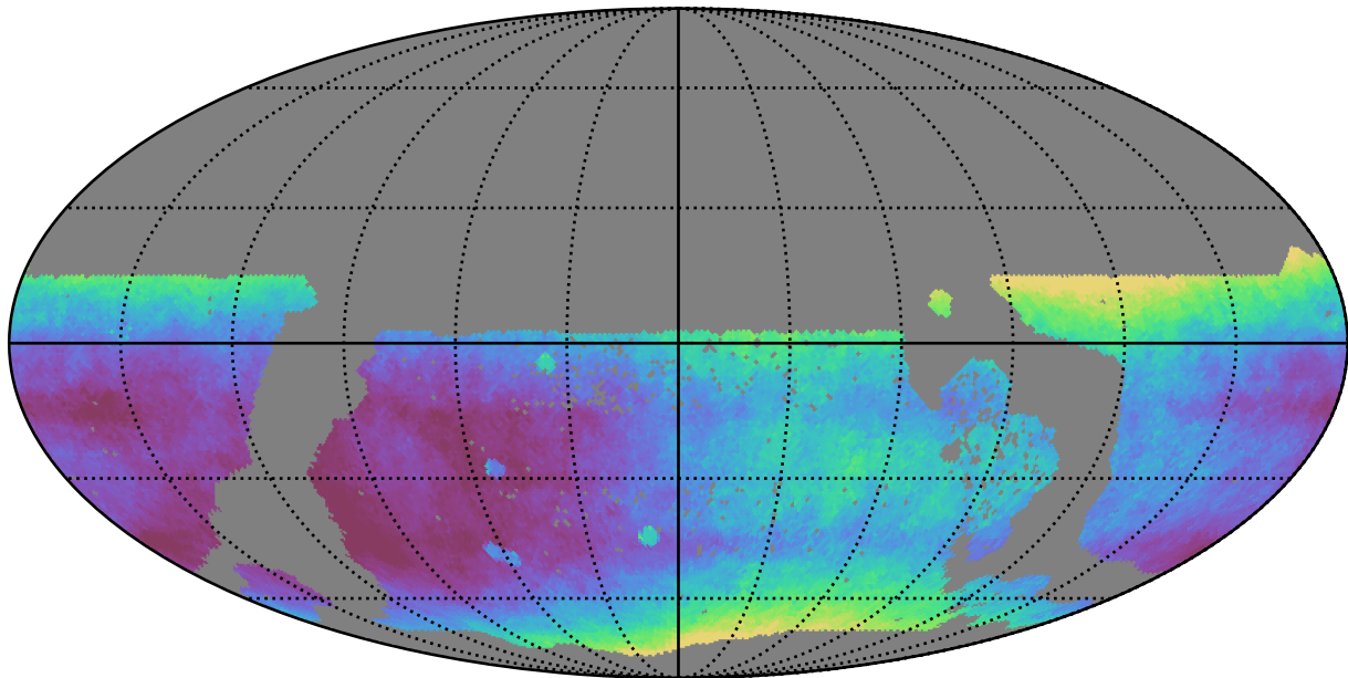
too_elab_r32_d2_gz_v3.4_10yrs WFD all bands: Median seeingEff
