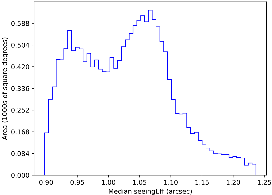
too_elab_r32_d2_gz_v3.4_10yrs WFD all bands: Median seeingEff
