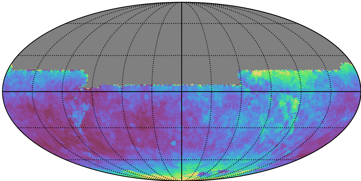
too_elab_r32_d2_gz_v3.4_10yrs All sky y band: Median seeingEff
