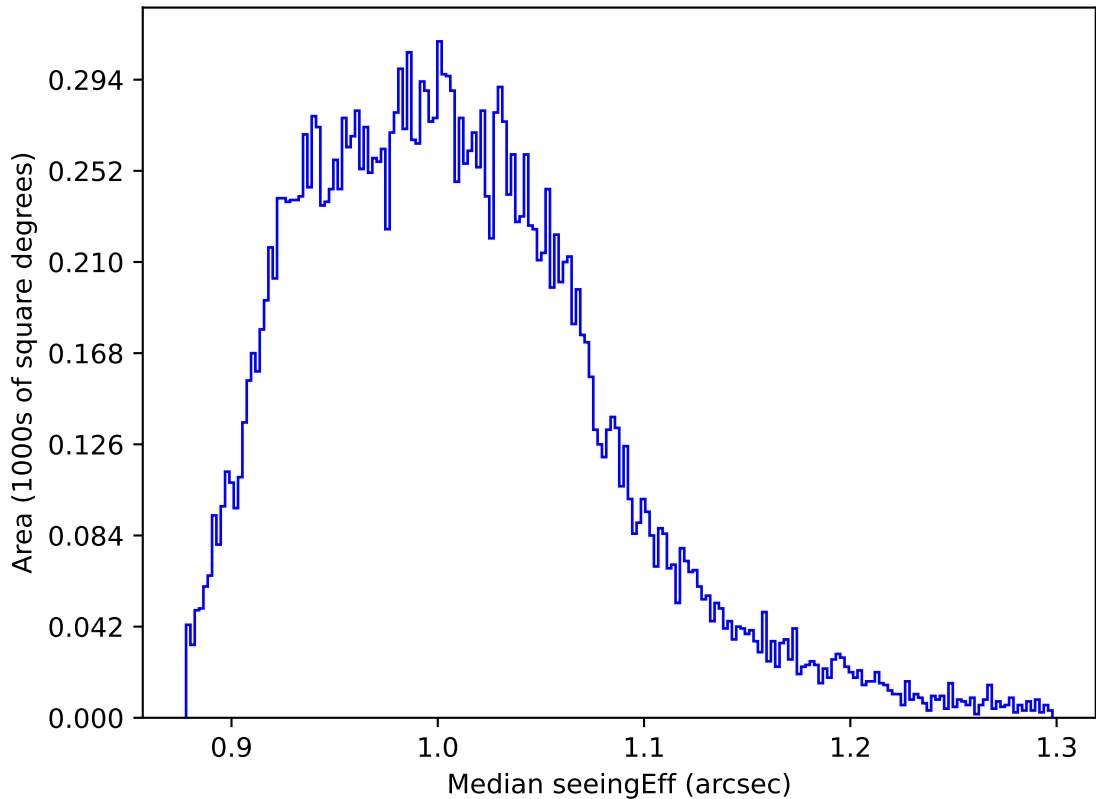
too_elab_r32_d2_gz_v3.4_10yrs All sky y band: Median seeingEff
