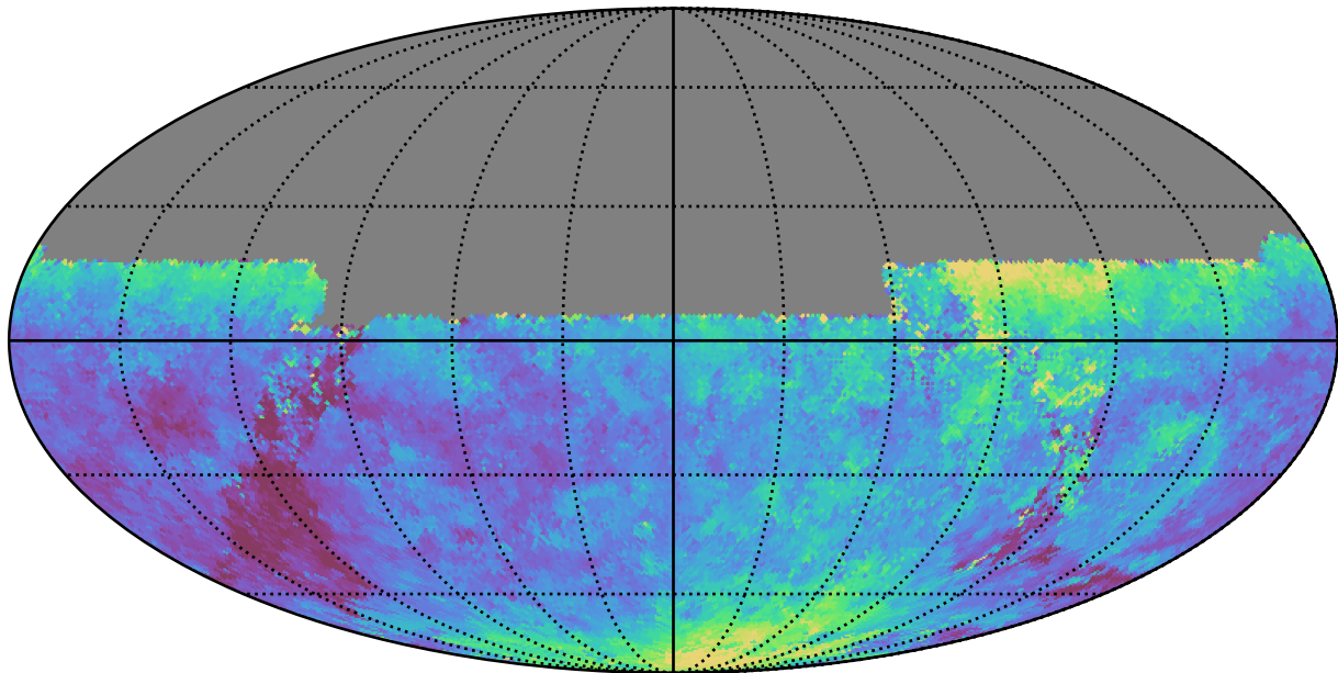
too_elab_r32_d2_gz_v3.4_10yrs All sky u band: Median seeingEff
