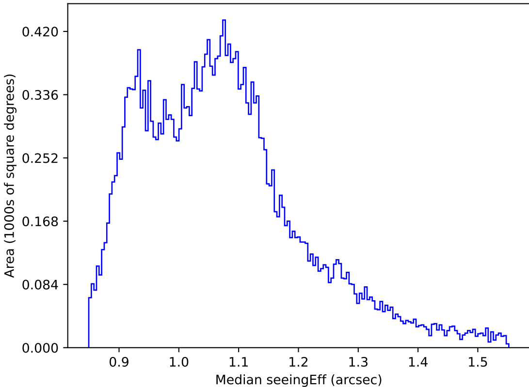
too_elab_r32_d2_gz_v3.4_10yrs All sky r band: Median seeingEff
