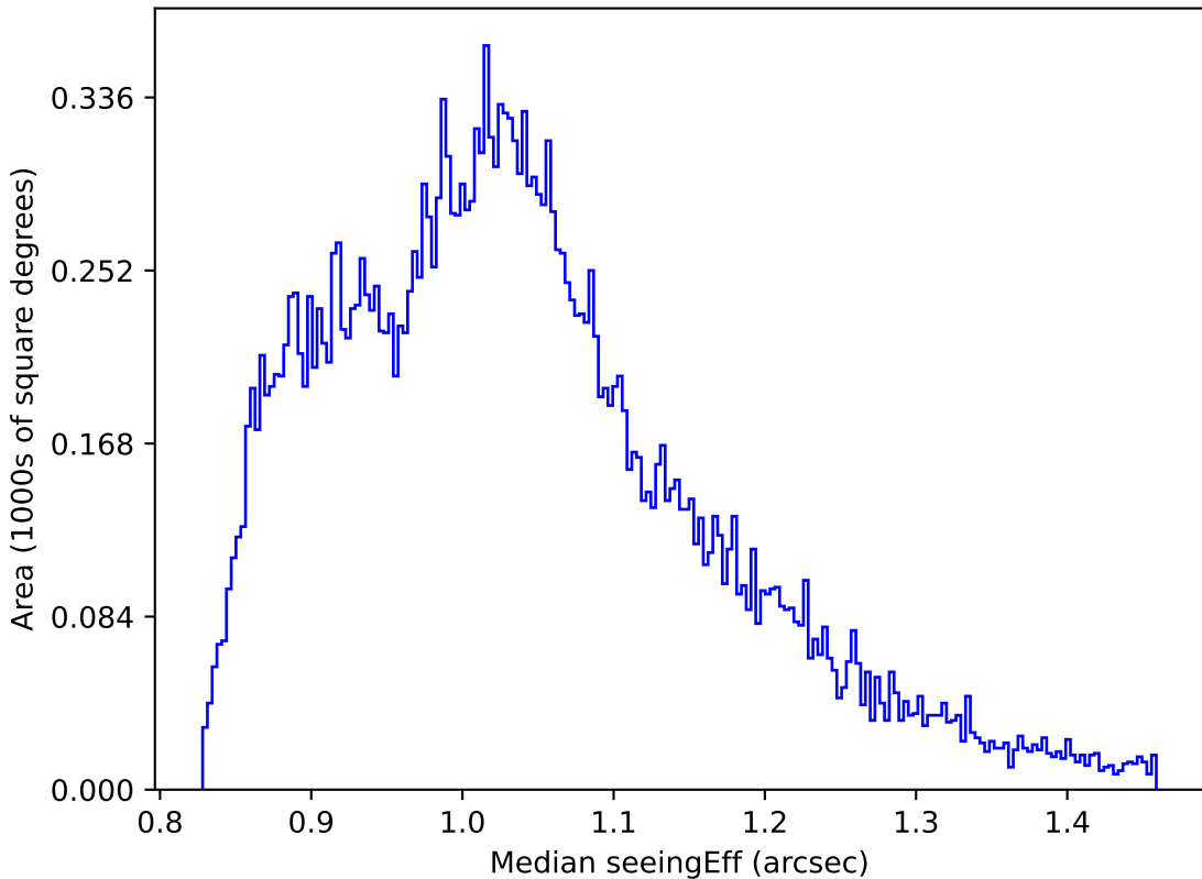
too_elab_r32_d2_gz_v3.4_10yrs All sky i band: Median seeingEff
