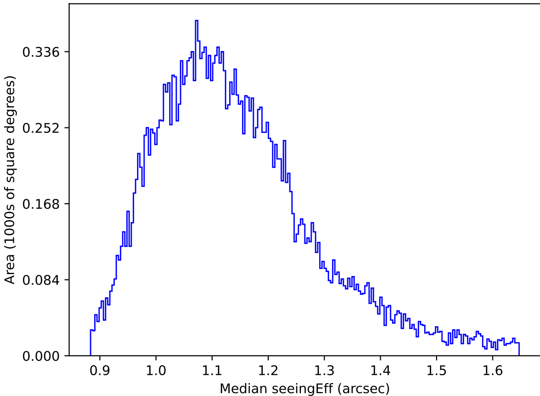
too_elab_r32_d2_gz_v3.4_10yrs All sky g band: Median seeingEff
