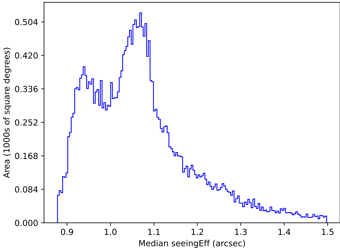
too_elab_r32_d2_gz_v3.4_10yrs All sky all bands: Median seeingEff
