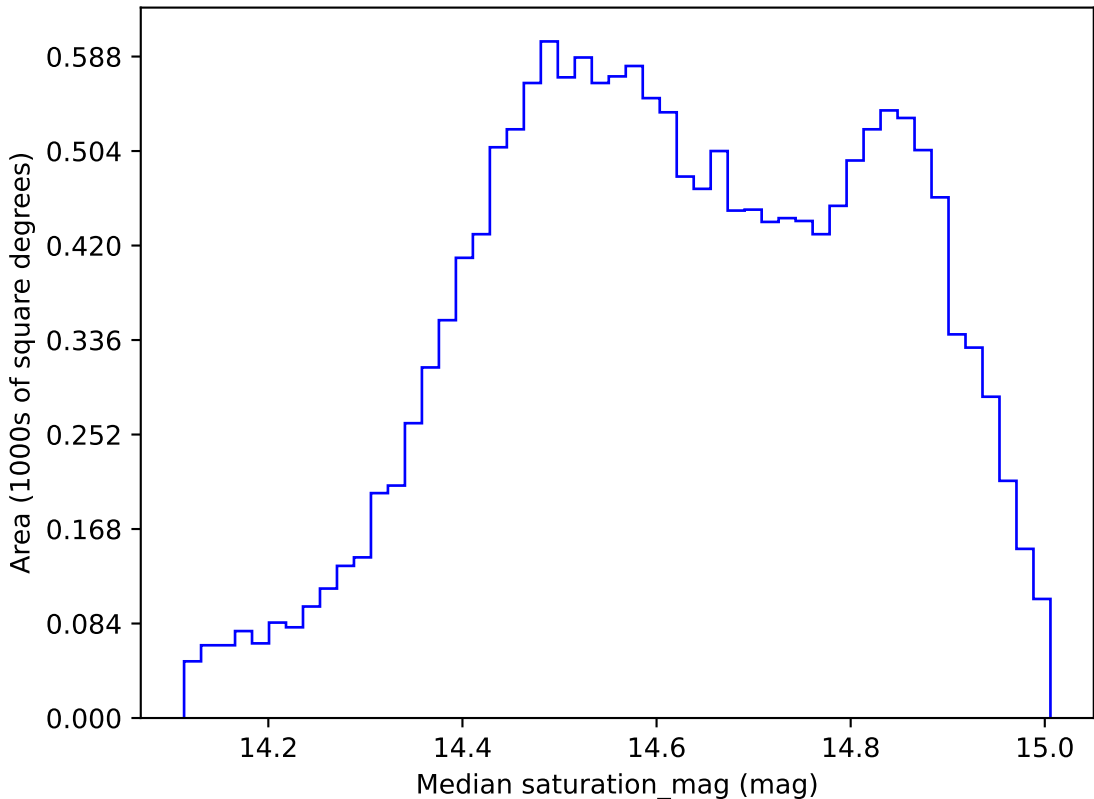
too_elab_r32_d2_gz_v3.4_10yrs WFD r band: Median saturation_mag
