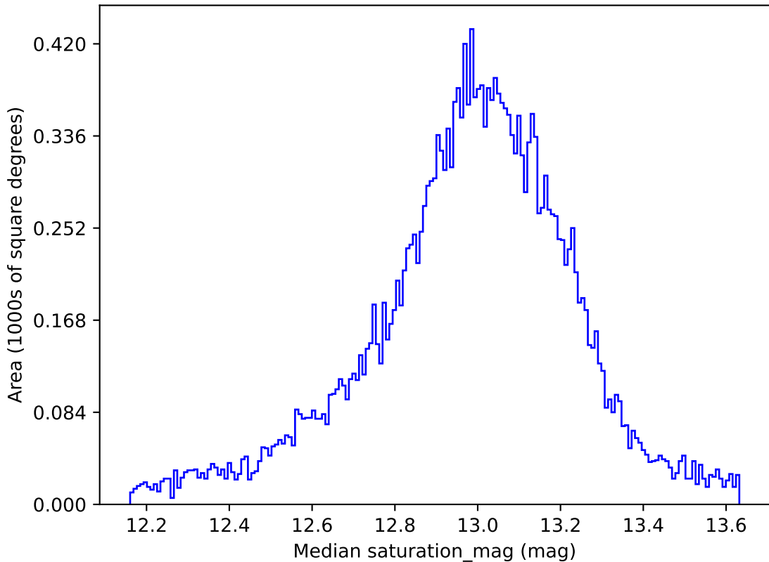
too_elab_r32_d2_gz_v3.4_10yrs All sky u band: Median saturation_mag
