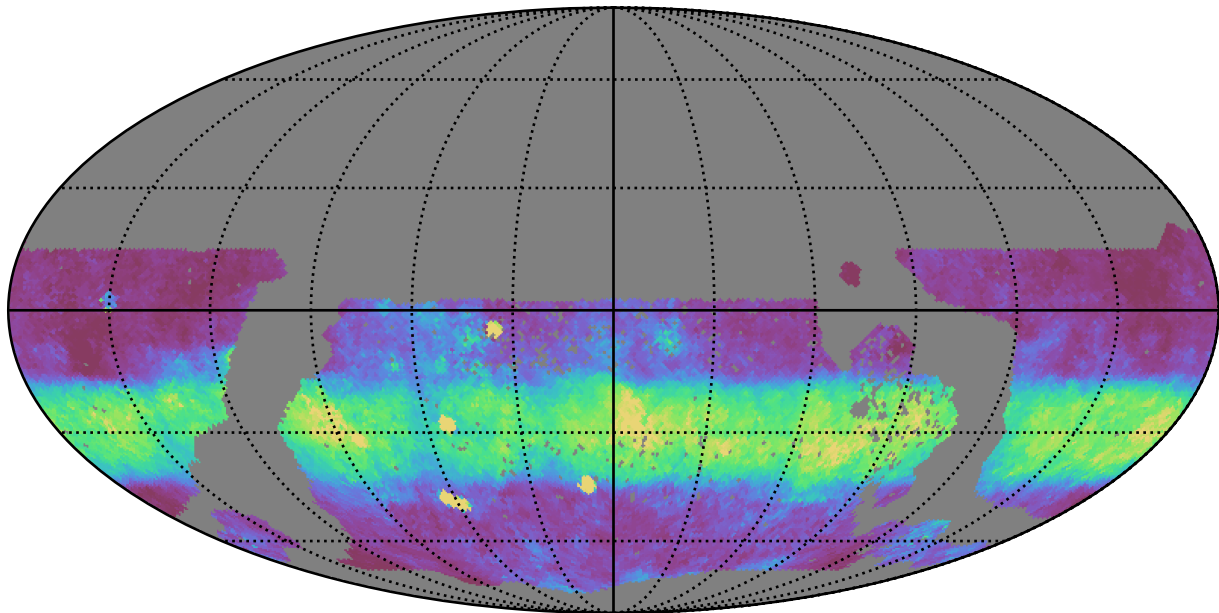
too_elab_r32_d2_gz_v3.4_10yrs WFD z band: Median normairmass
