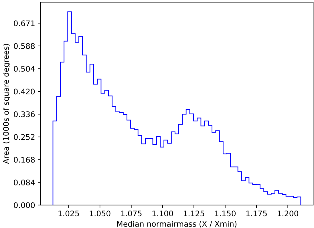
too_elab_r32_d2_gz_v3.4_10yrs WFD u band: Median normairmass
