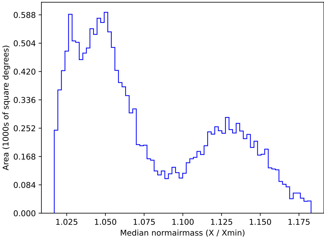
too_elab_r32_d2_gz_v3.4_10yrs WFD r band: Median normairmass
