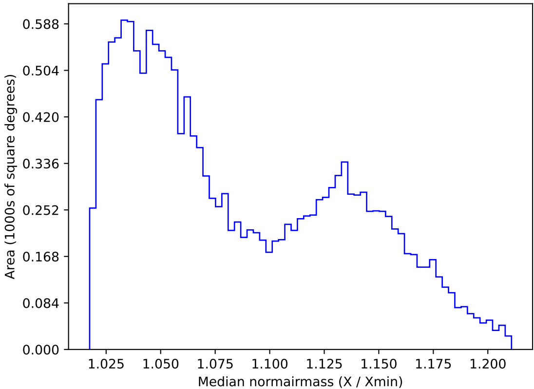
too_elab_r32_d2_gz_v3.4_10yrs WFD g band: Median normairmass
