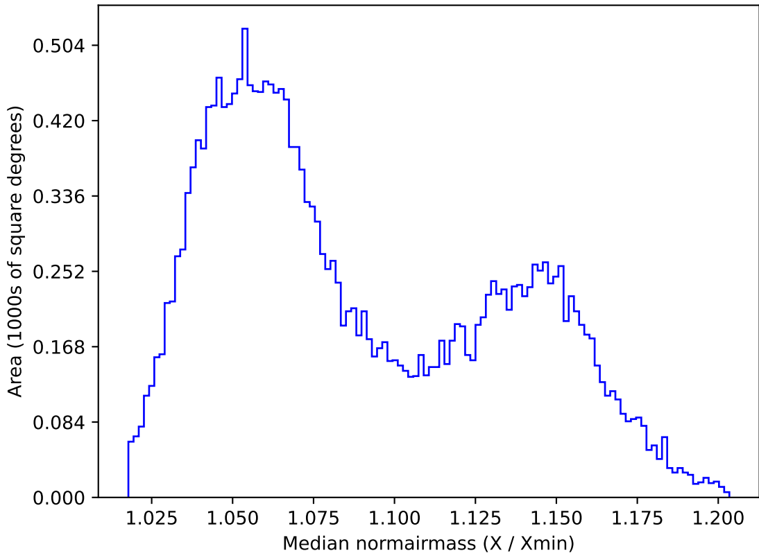
too_elab_r32_d2_gz_v3.4_10yrs All sky y band: Median normairmass
