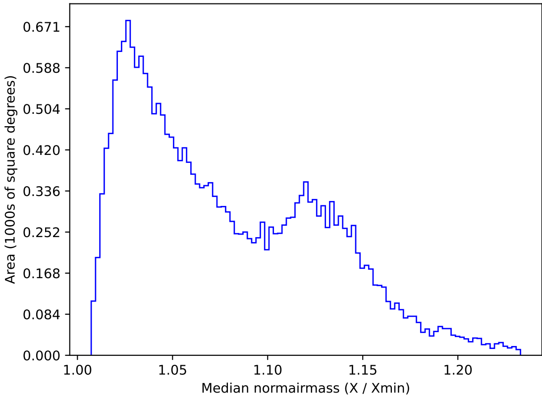
too_elab_r32_d2_gz_v3.4_10yrs All sky u band: Median normairmass
