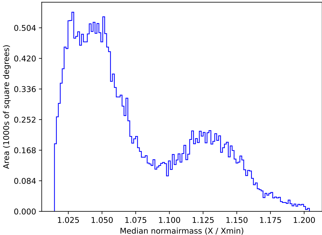
too_elab_r32_d2_gz_v3.4_10yrs All sky r band: Median normairmass
