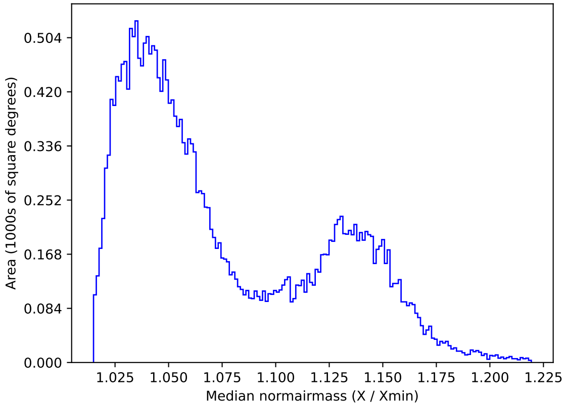
too_elab_r32_d2_gz_v3.4_10yrs All sky i band: Median normairmass
