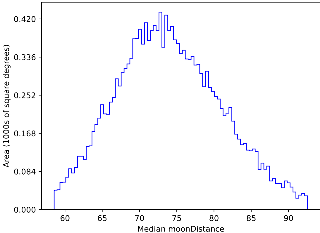
too_elab_r32_d2_gz_v3.4_10yrs WFD z band: Median moonDistance
