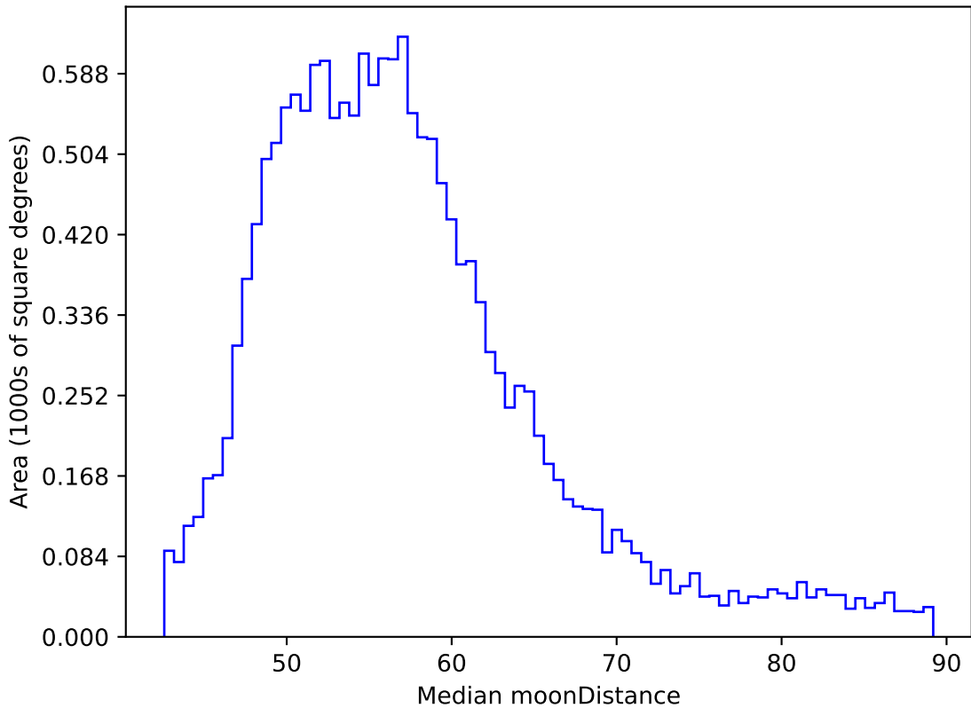
too_elab_r32_d2_gz_v3.4_10yrs WFD y band: Median moonDistance
