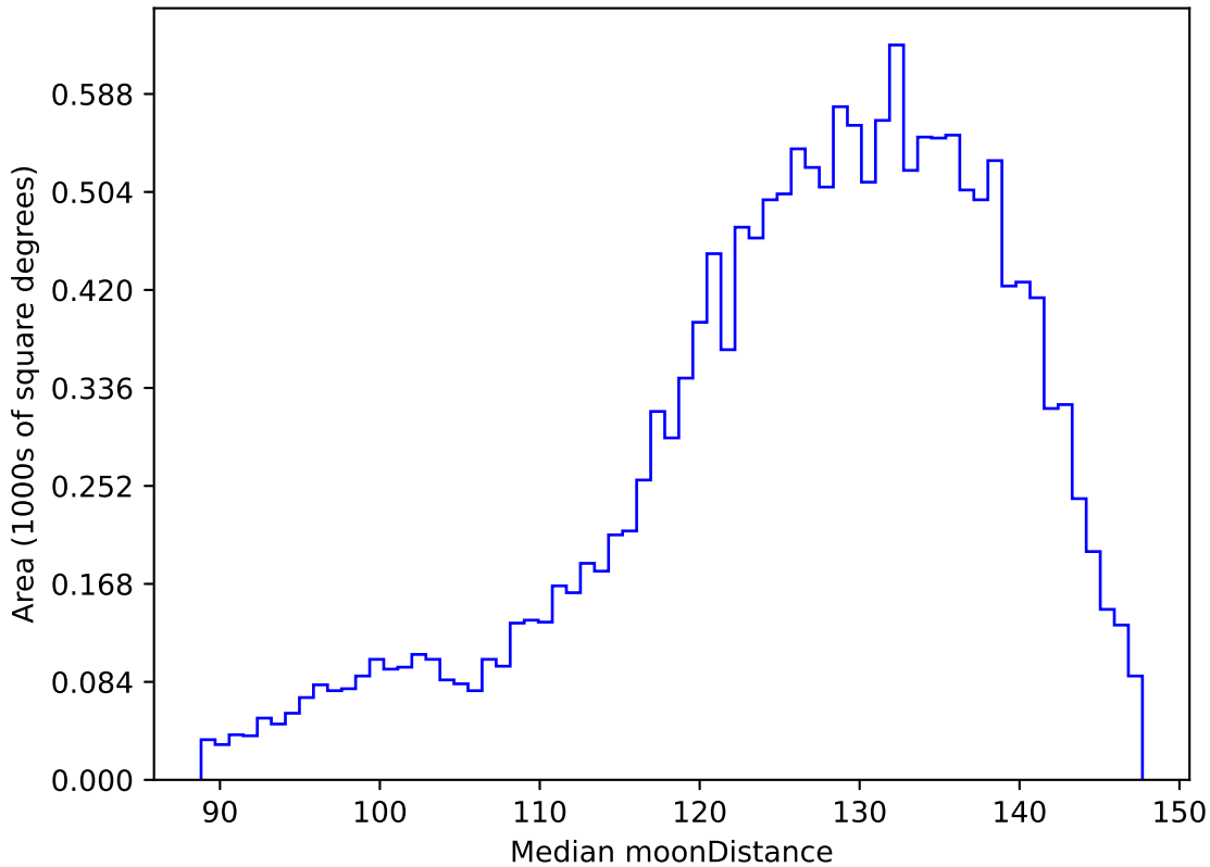
too_elab_r32_d2_gz_v3.4_10yrs WFD u band: Median moonDistance
