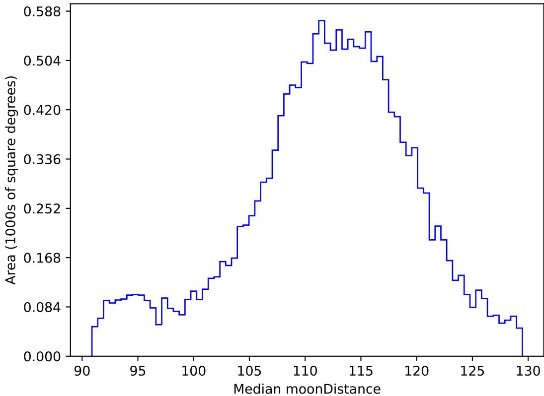
too_elab_r32_d2_gz_v3.4_10yrs WFD r band: Median moonDistance
