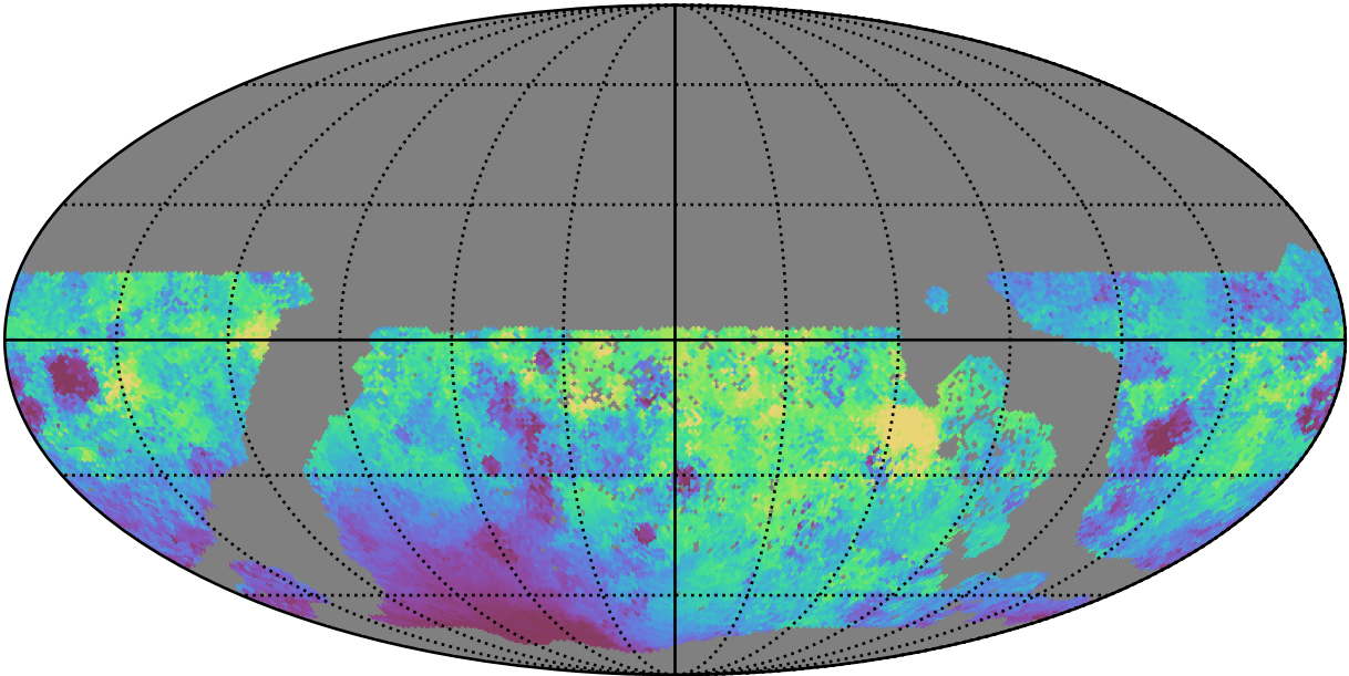
too_elab_r32_d2_gz_v3.4_10yrs WFD g band: Median moonDistance
