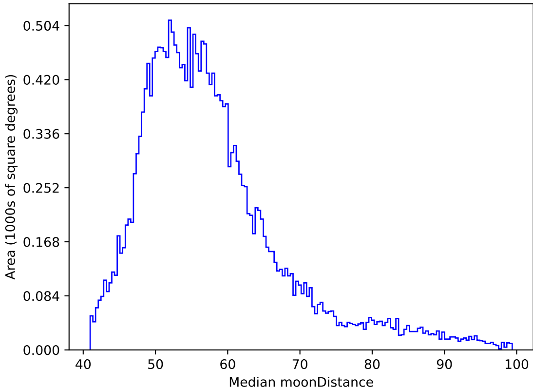
too_elab_r32_d2_gz_v3.4_10yrs All sky y band: Median moonDistance
