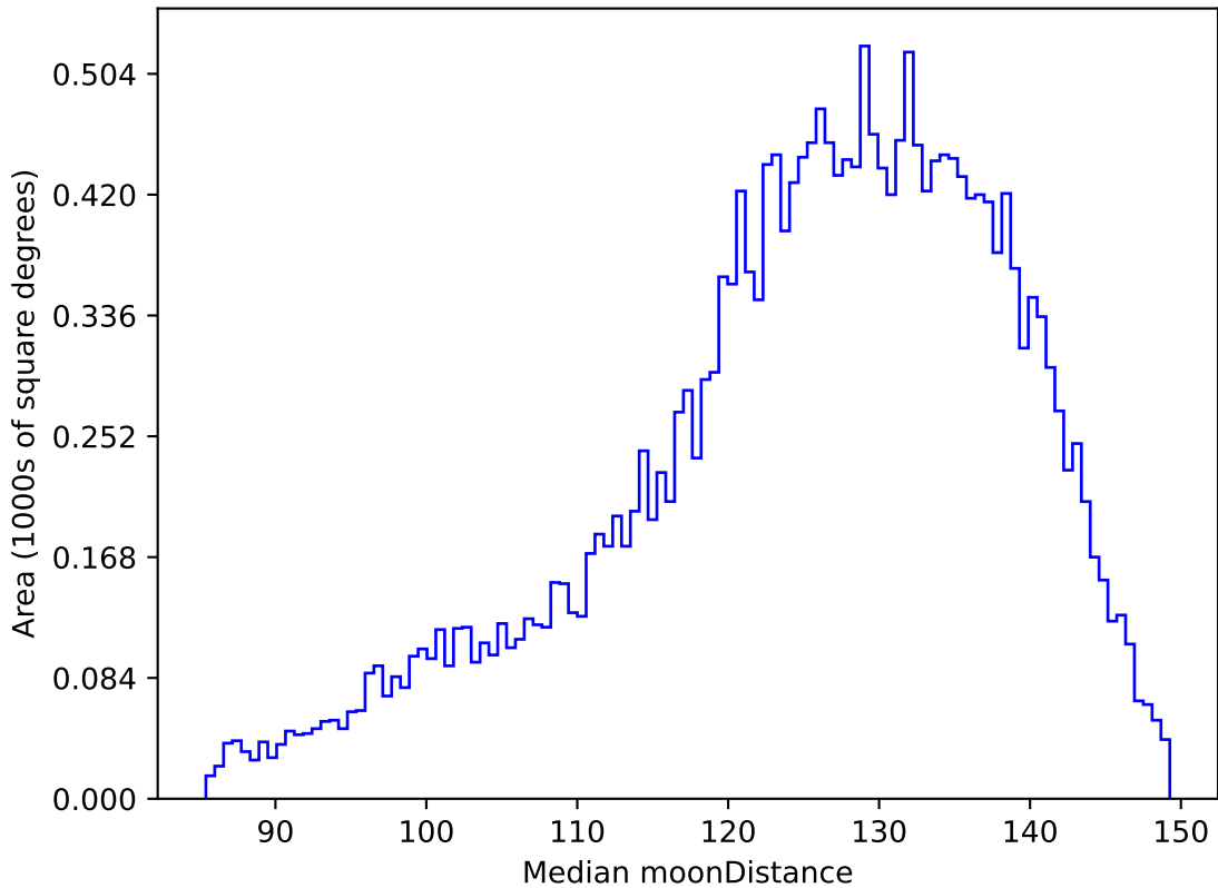
too_elab_r32_d2_gz_v3.4_10yrs All sky u band: Median moonDistance
