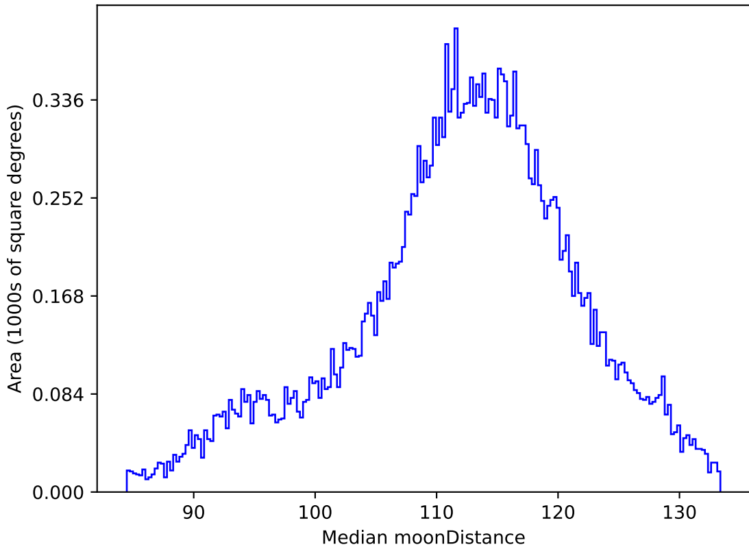
too_elab_r32_d2_gz_v3.4_10yrs All sky r band: Median moonDistance
