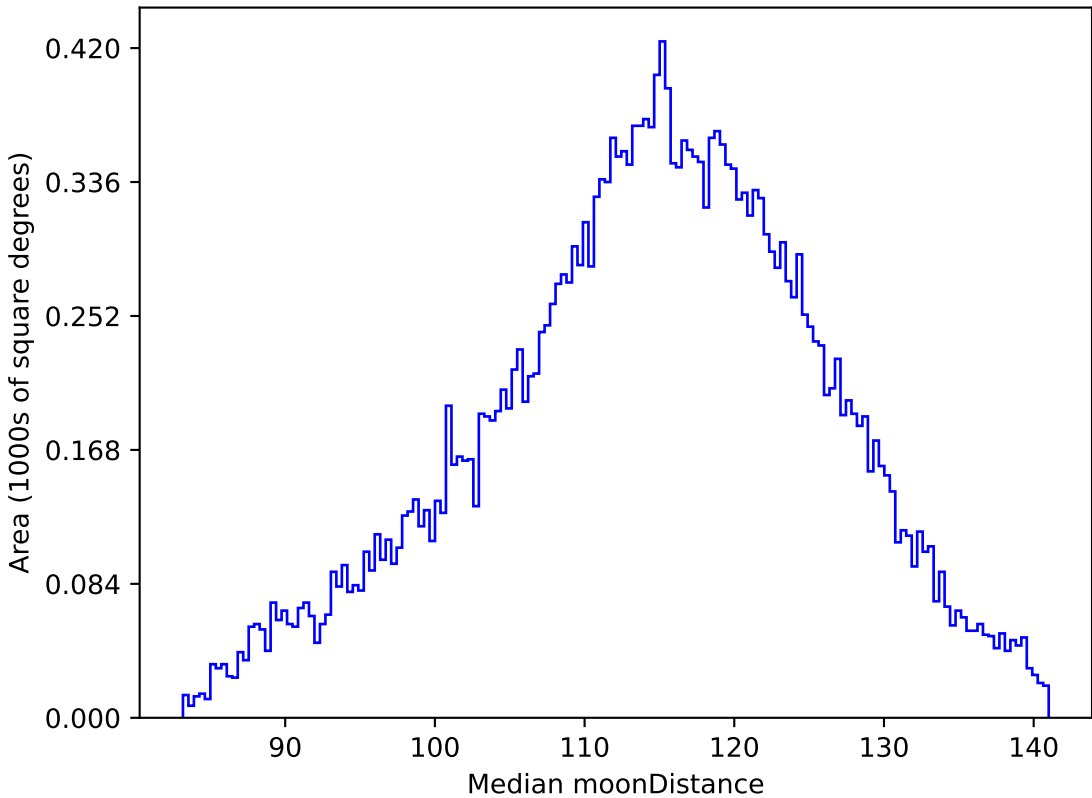
too_elab_r32_d2_gz_v3.4_10yrs All sky g band: Median moonDistance
