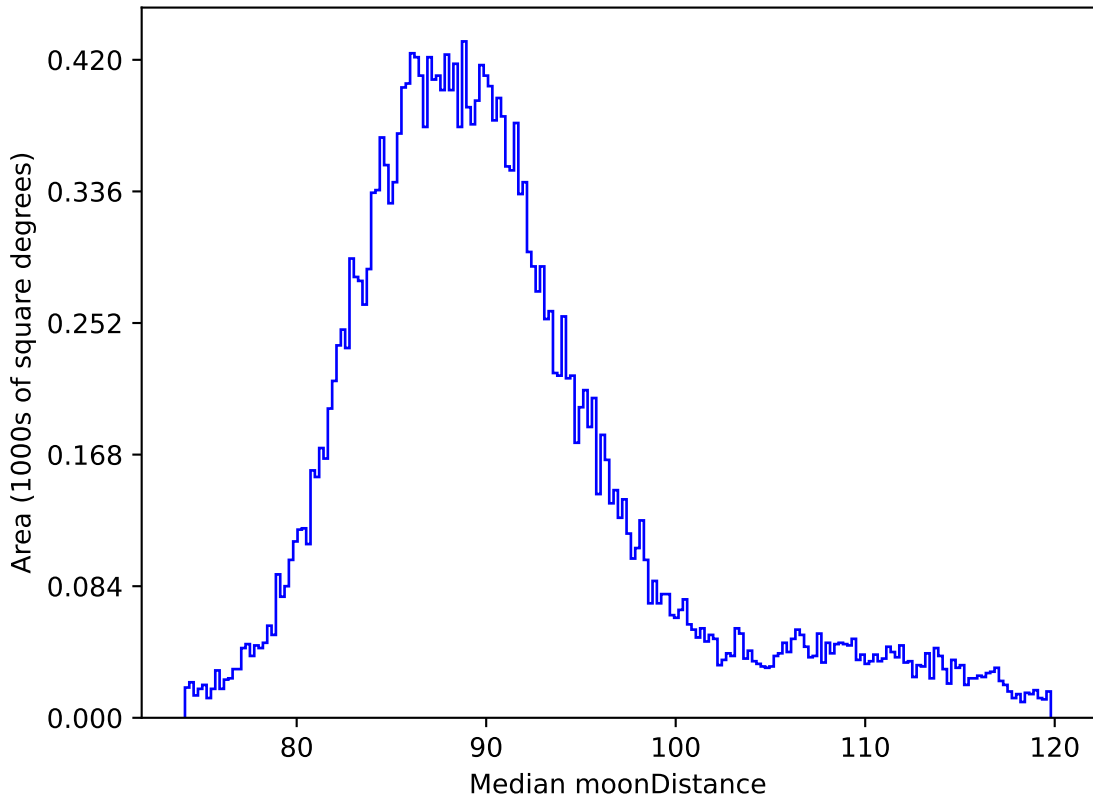
too_elab_r32_d2_gz_v3.4_10yrs All sky all bands: Median moonDistance
