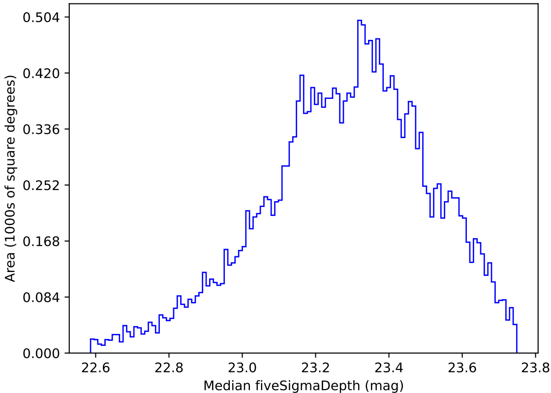
too_elab_r32_d2_gz_v3.4_10yrs Yr 1 u band: Median fiveSigmaDepth
