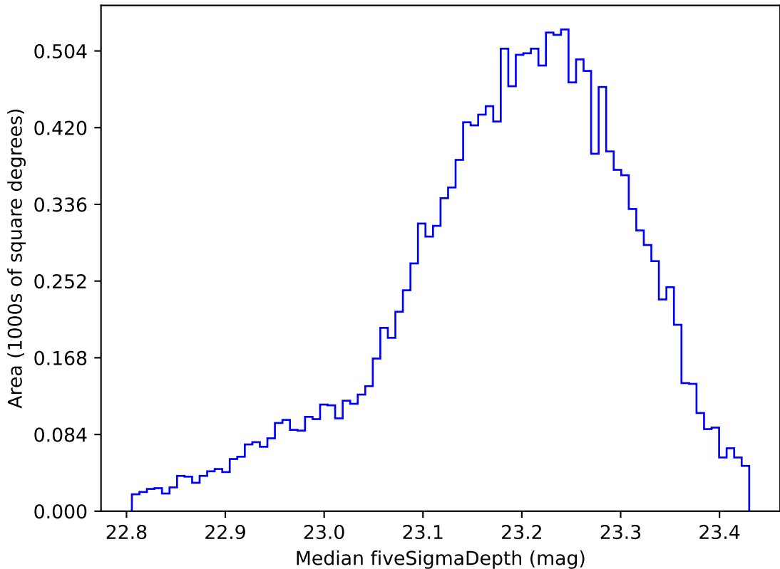
too_elab_r32_d2_gz_v3.4_10yrs WFD u band: Median fiveSigmaDepth
