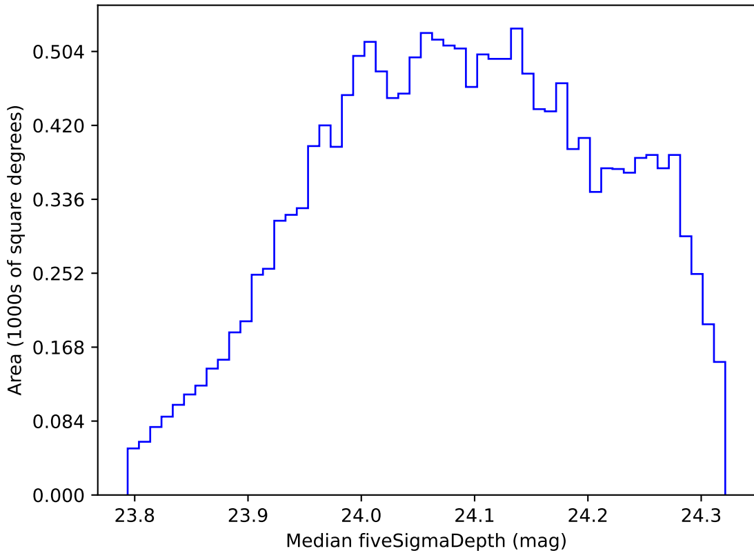
too_elab_r32_d2_gz_v3.4_10yrs WFD r band: Median fiveSigmaDepth
