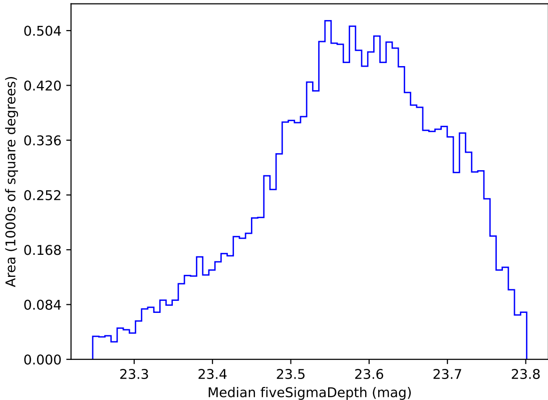
too_elab_r32_d2_gz_v3.4_10yrs WFD i band: Median fiveSigmaDepth
