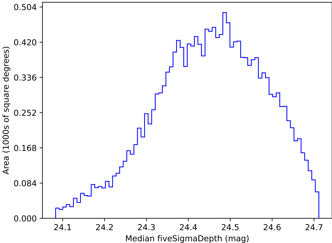
too_elab_r32_d2_gz_v3.4_10yrs WFD g band: Median fiveSigmaDepth
