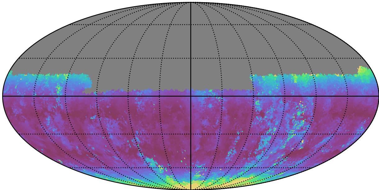
too_elab_r32_d2_gz_v3.4_10yrs Yr 1 u band: Median airmass
