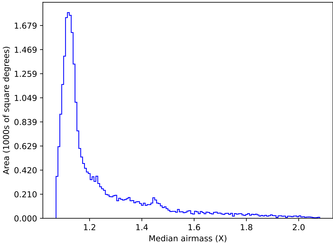
too_elab_r32_d2_gz_v3.4_10yrs Yr 1 all bands: Median airmass
