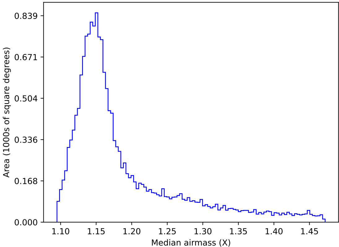
too_elab_r32_d2_gz_v3.4_10yrs WFD y band: Median airmass
